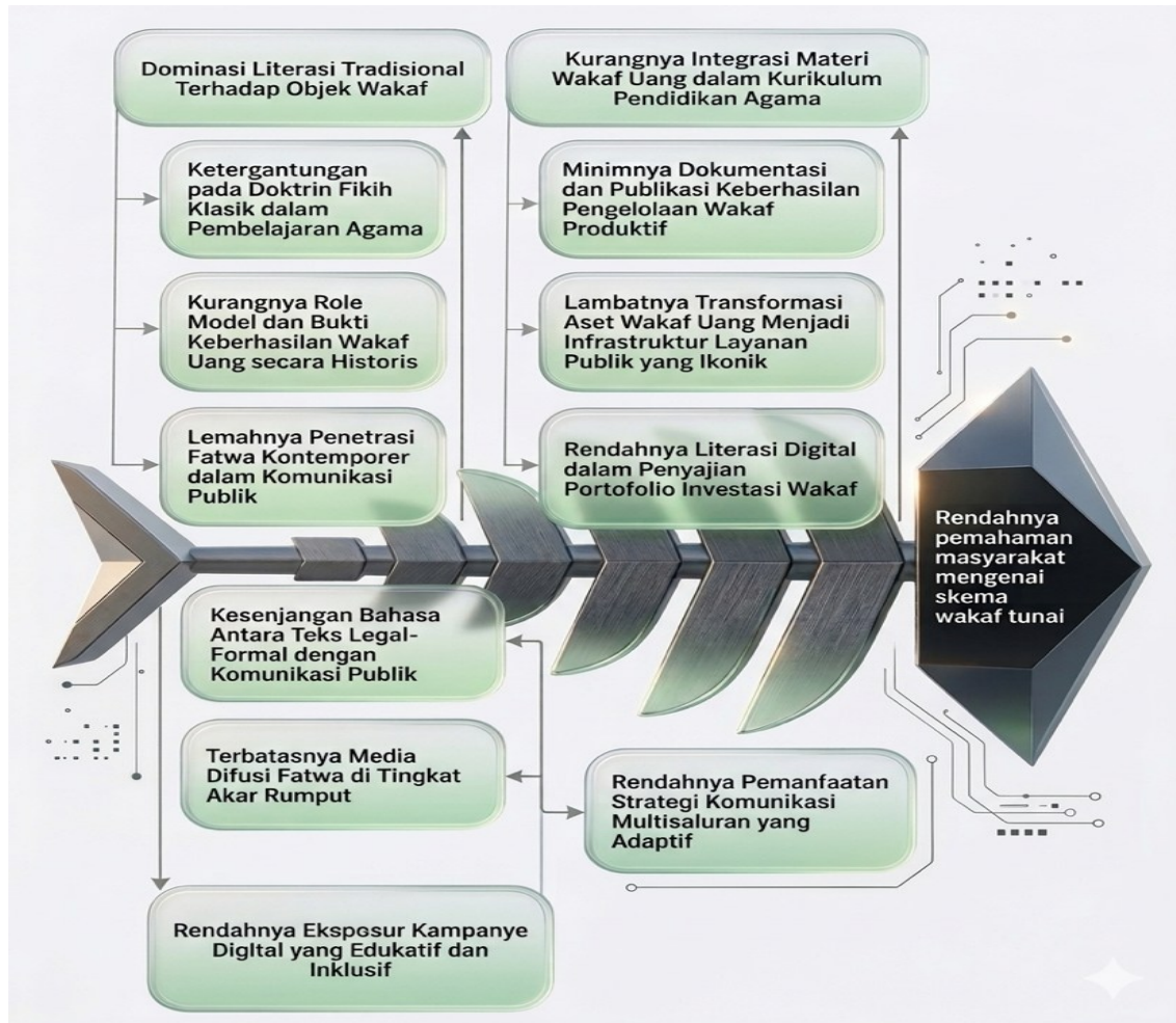
Gambar 1. Diagram Fishbone
