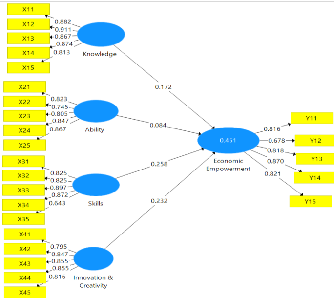
Figure 2. Outer Models
